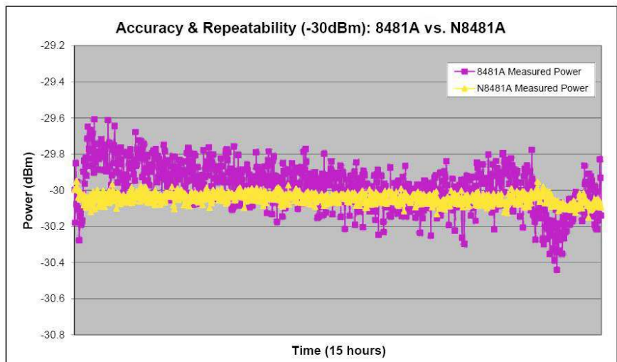
Figure 2. Power measurement comparison between the N8481A and legacy 8481A power sensor
